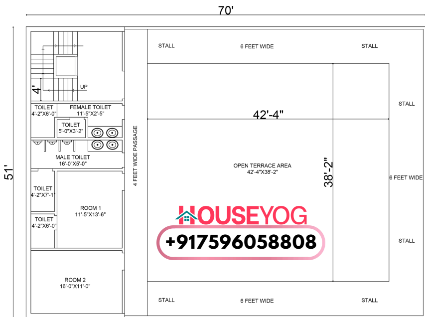
Roof Top Plan
